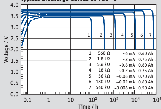
Typical Discharge Curves at +85 °C
